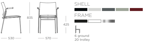
ARM CHAIR 4 LEG METAL FRAME KAVAC
