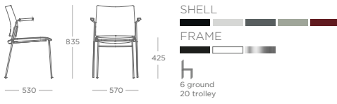
ARM CHAIR 4 LEG METAL FRAME KAVAC.PU
