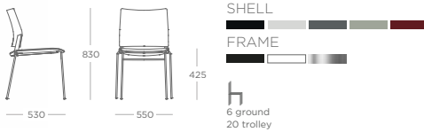
SIDE CHAIR 4 LEG METAL FRAME KAVSC.PU
