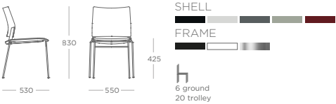
SIDE CHAIR 4 LEG METAL FRAME KAVSC
