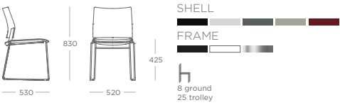
SIDE CHAIR METAL SLED FRAME KAVSC.S
