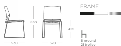
SIDE CHAIR METAL SLED FRAME KAVSC.S.U
