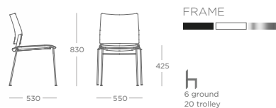
SIDE CHAIR 4 LEG METAL FRAME KAVSC.U
