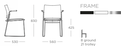
ARM CHAIR METAL SLED FRAME KAVAC.S.U
