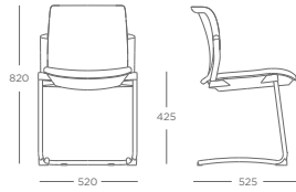
CANTILEVER FRAME OPP.CF
